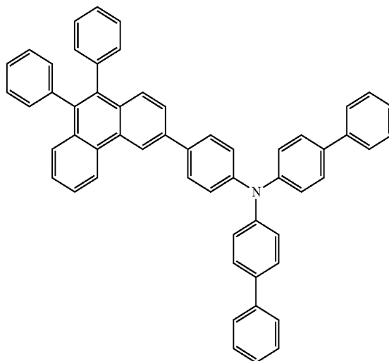
chemical formula 1-6
