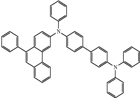
chemical formula 2-11
