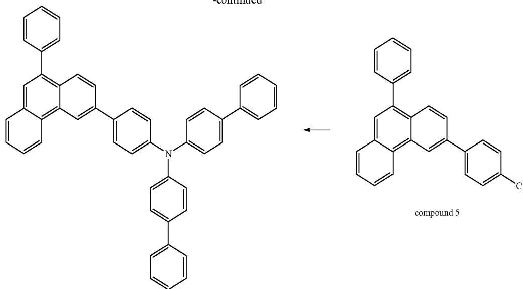
chemical formula 1-7
