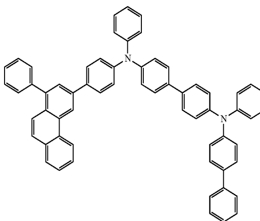
chemical formula 2-29
