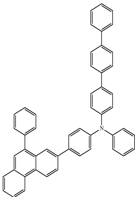
chemical formula 1-15
