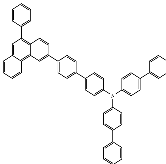
chemical formula 1-12
