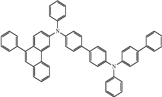
chemical formula 2-12
