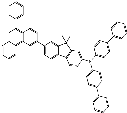
chemical formula 1-14
