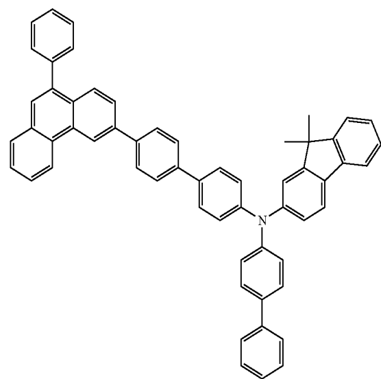
chemical formula 1-13
