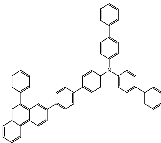
chemical formula 1-18
