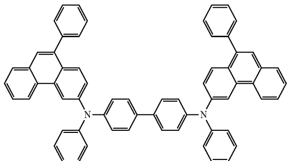
chemical formula 2-5
