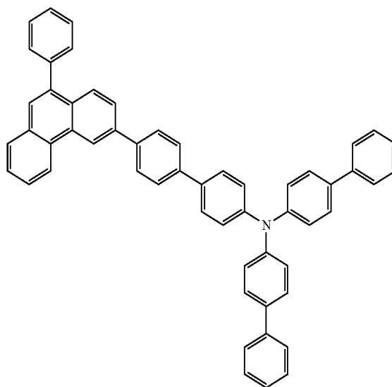
chemical formula 1-11
