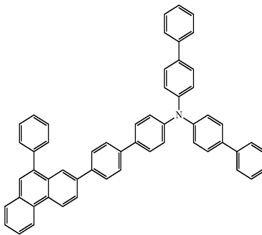
chemical formula 1-18
