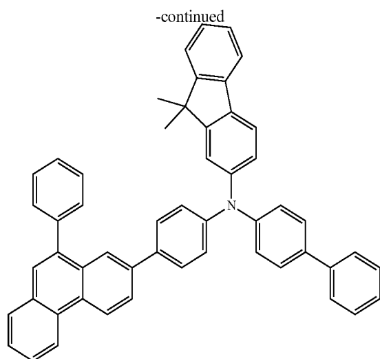
chemical formula 1-4
