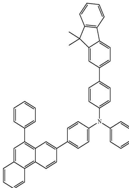
chemical formula 1-17
