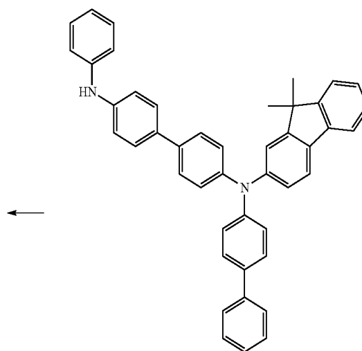
compound 4
