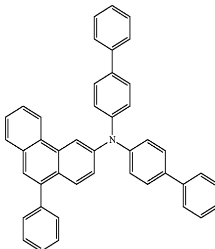
chemical formula 1-23
