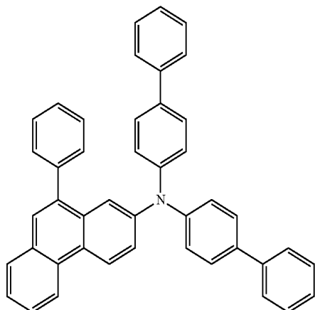
chemical formula 1-21
