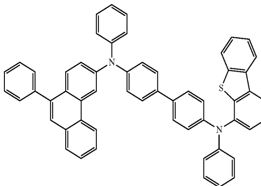
chemical formula 2-21
