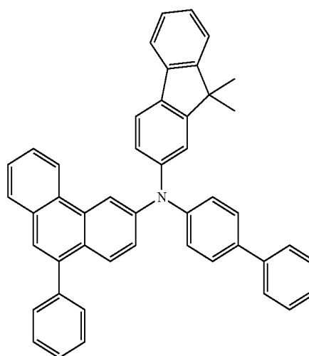
chemical formula 1-24
