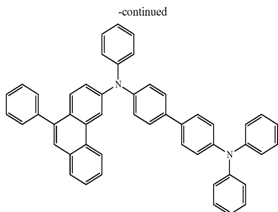
chemical formula 2-11
