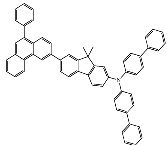
chemical formula 1-13
