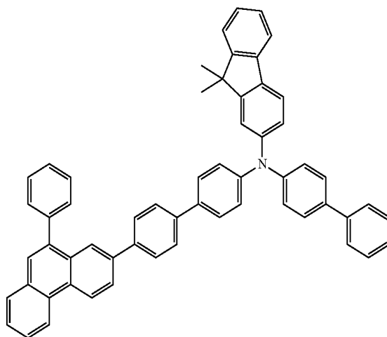
chemical formula 1-18
