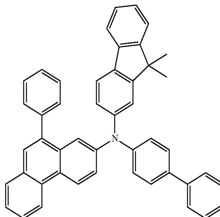
chemical formula 1-23
