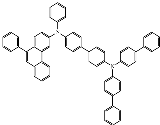
chemical formula 2-13
