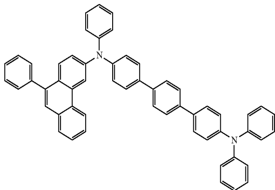
chemical formula 2-16
