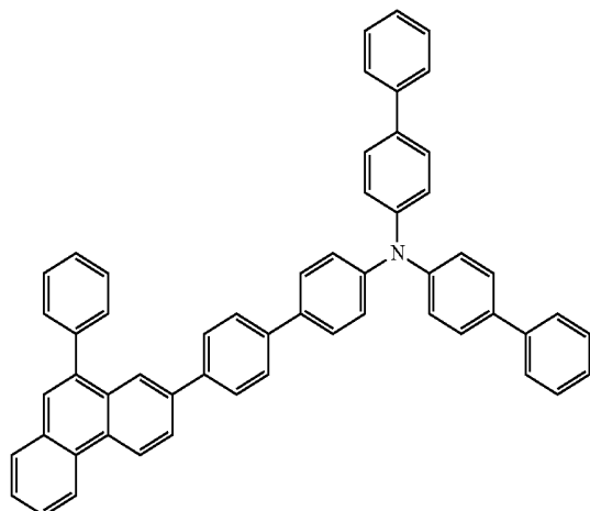
chemical formula 1-20
