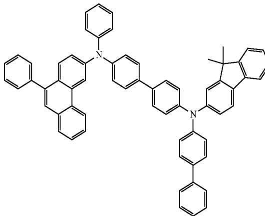
chemical formula 2-14
