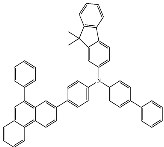
chemical formula 1-4
