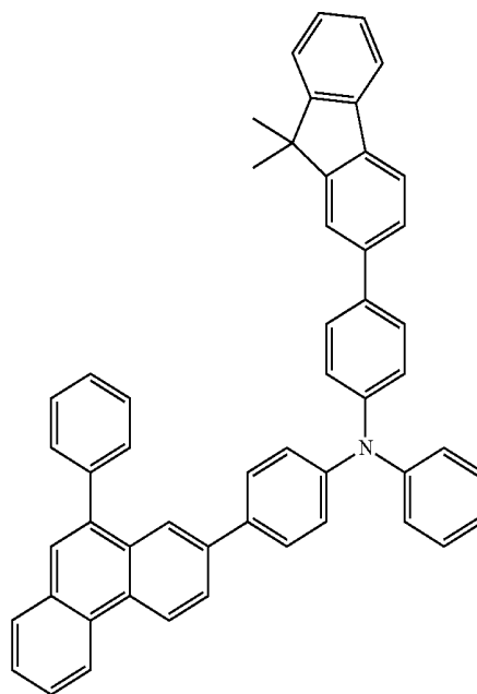
chemical formula 1-17
