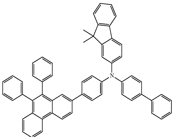
chemical formula 1-2
