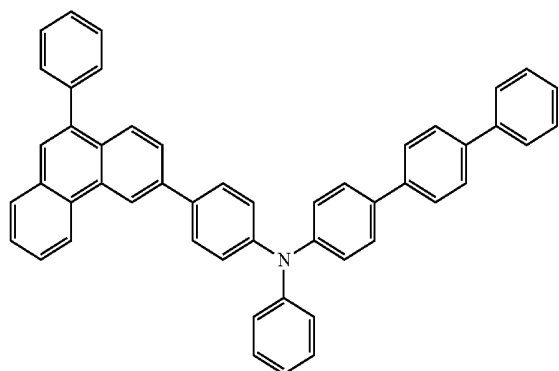
chemical formula 1-9
