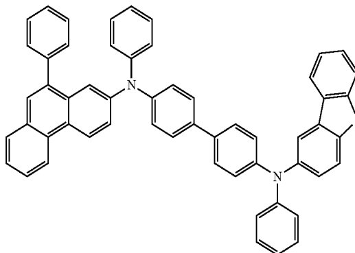
chemical formula 2-25
