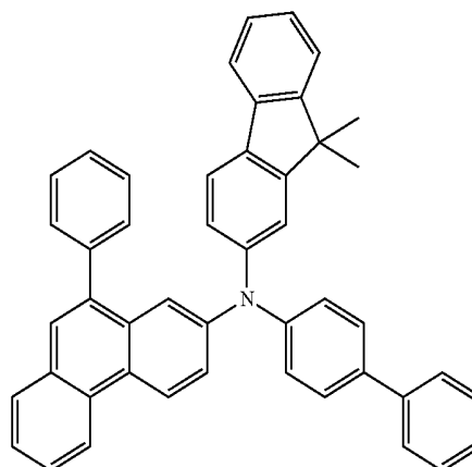
chemical formula 1-22
