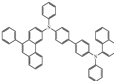
chemical formula 2-19
