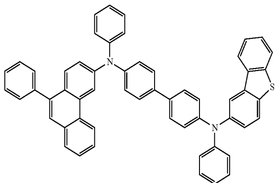
chemical formula 2-22
