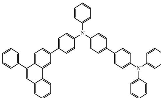
chemical formula 2-27
