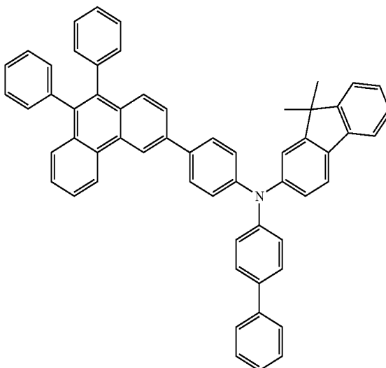
chemical formula 1-7
