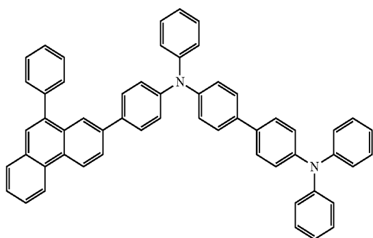
chemical formula 2-28
