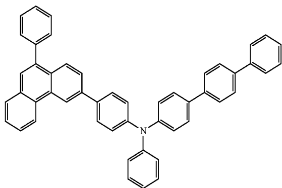
chemical formula 1-9
