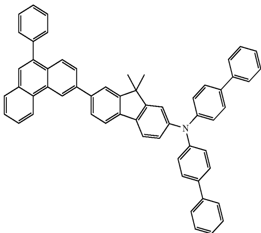
chemical formula 1-15
