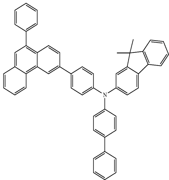
chemical formula 1-9
