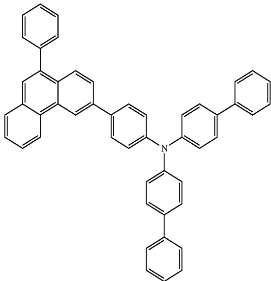
chemical formula 1-8
