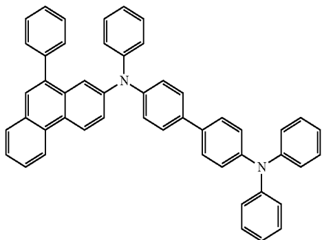
chemical formula 2-7
