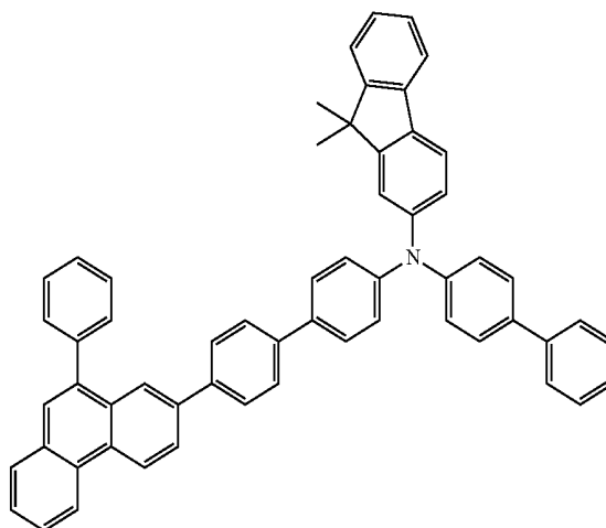
chemical formula 1-18
