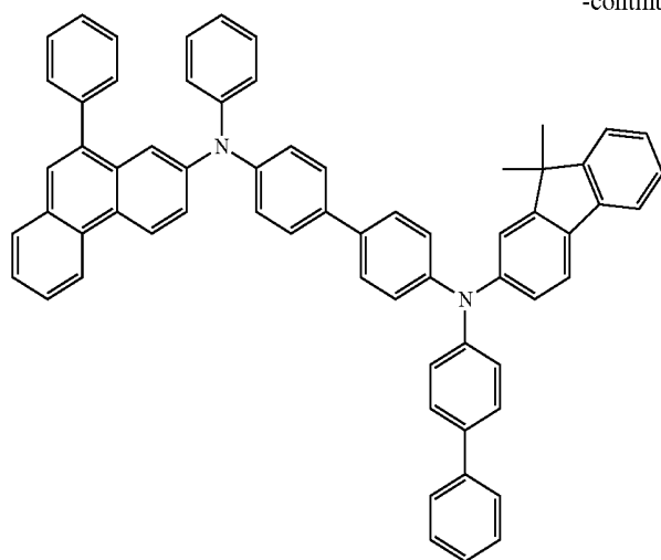
chemical formula 2-7
