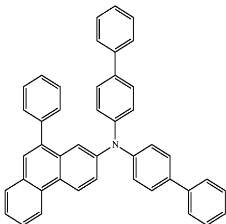
chemical formula 1-21
