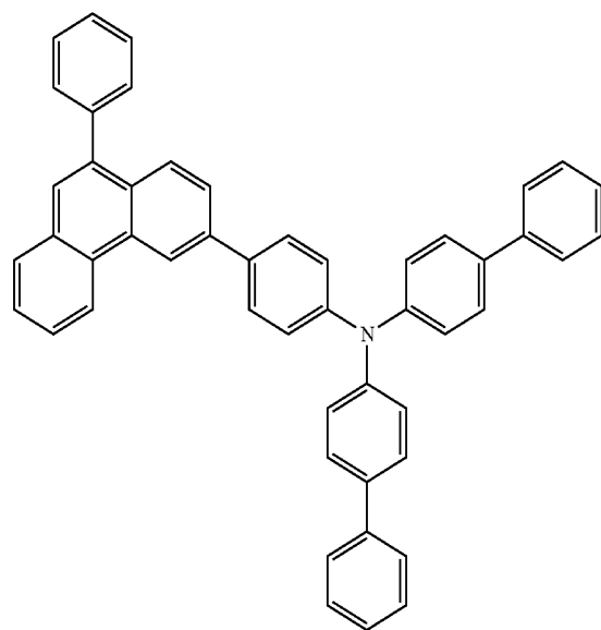
chemical formula 1-7
