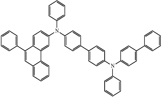
chemical formula 2-12
