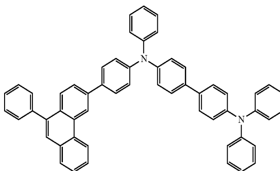
chemical formula 2-27
