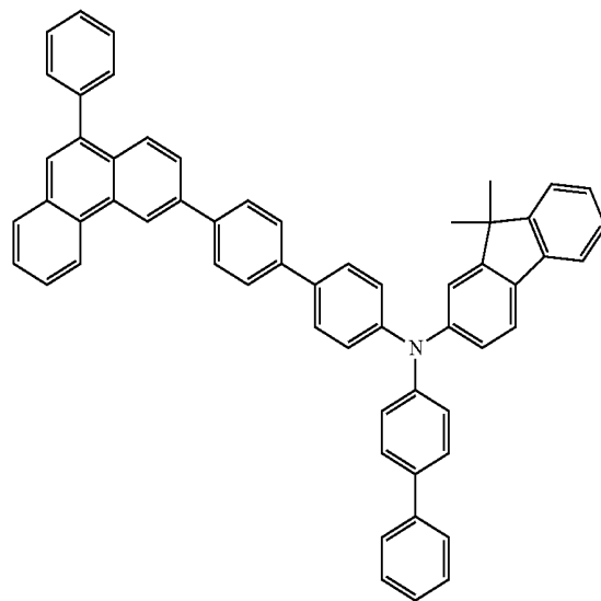
chemical formula 1-12
