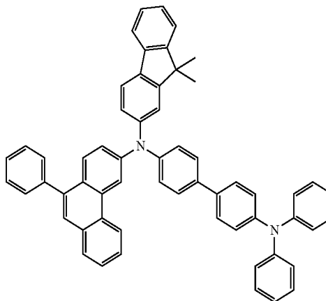
chemical formula 2-17
