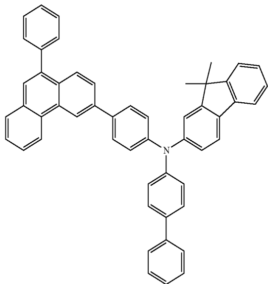
chemical formula 1-8
