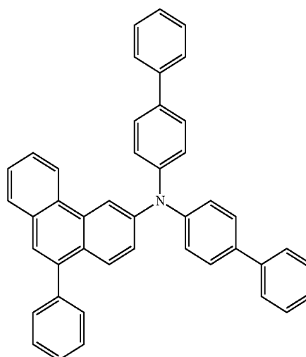
chemical formula 1-23
