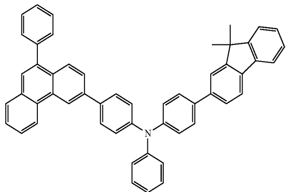
chemical formula 1-10
