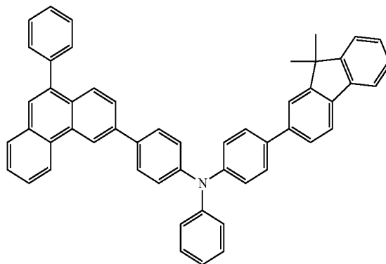
chemical formula 1-11
