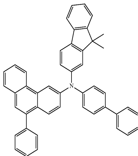
chemical formula 1-24
