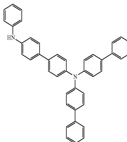
compound 4
